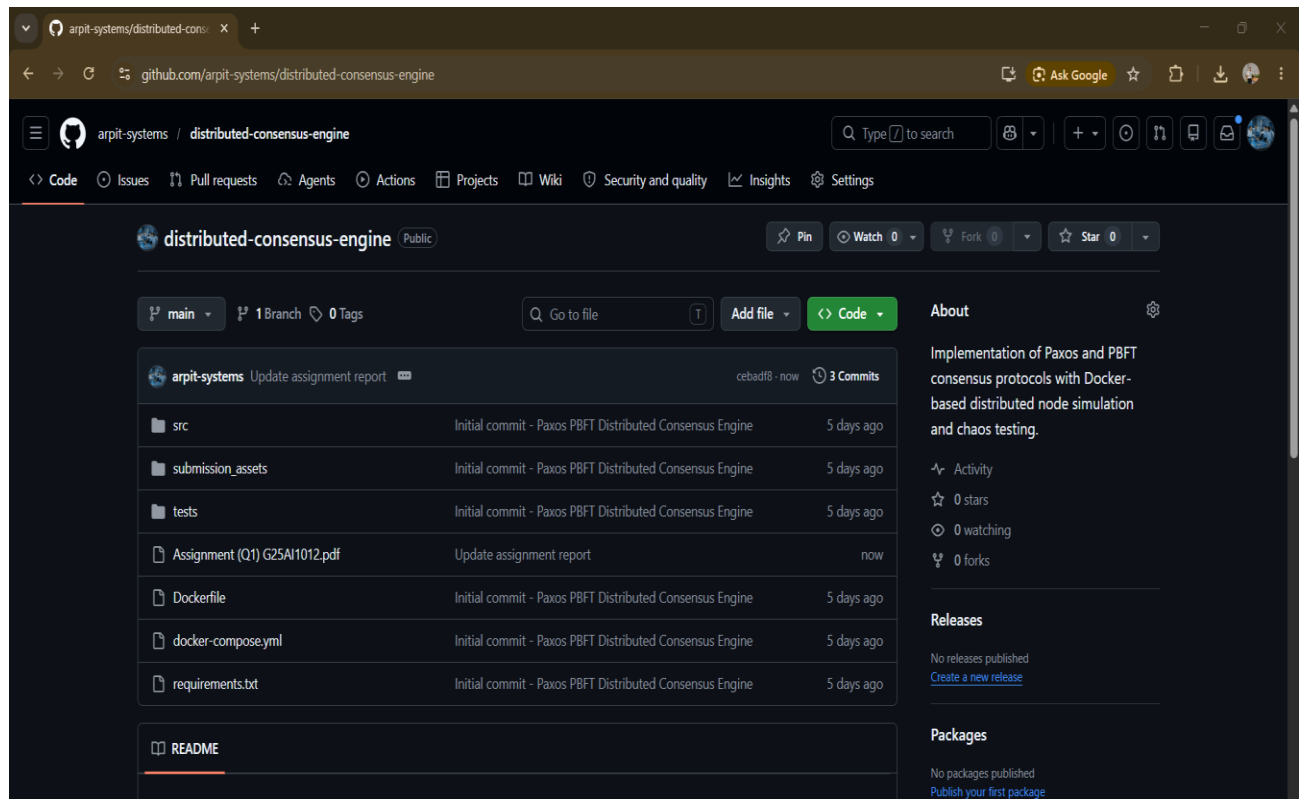
Figure 12: GitHub Repository
